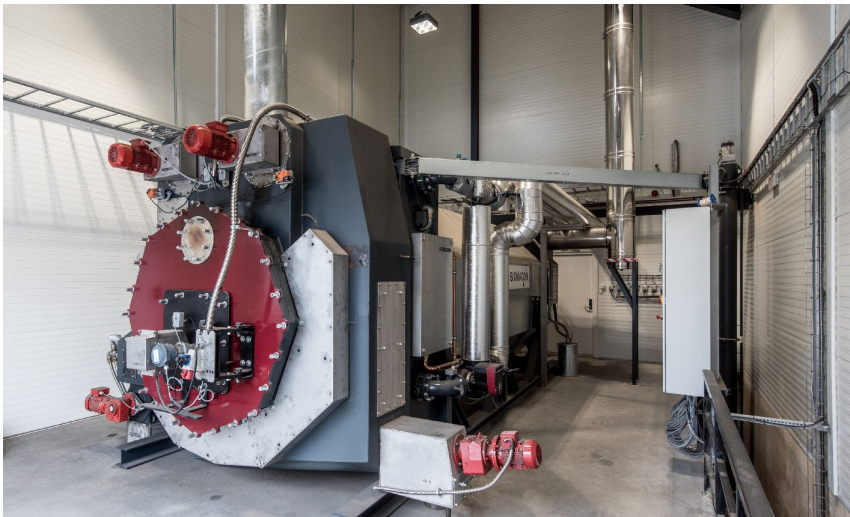
Abb. 03: Pyrolyseanlage Firma BIOMACON [Foto: Biomacon]
